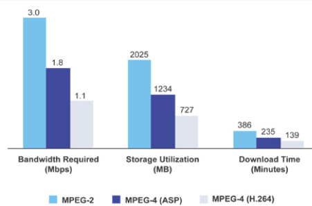
Performance comparison for 90-minute DVD-quality movie (1)
